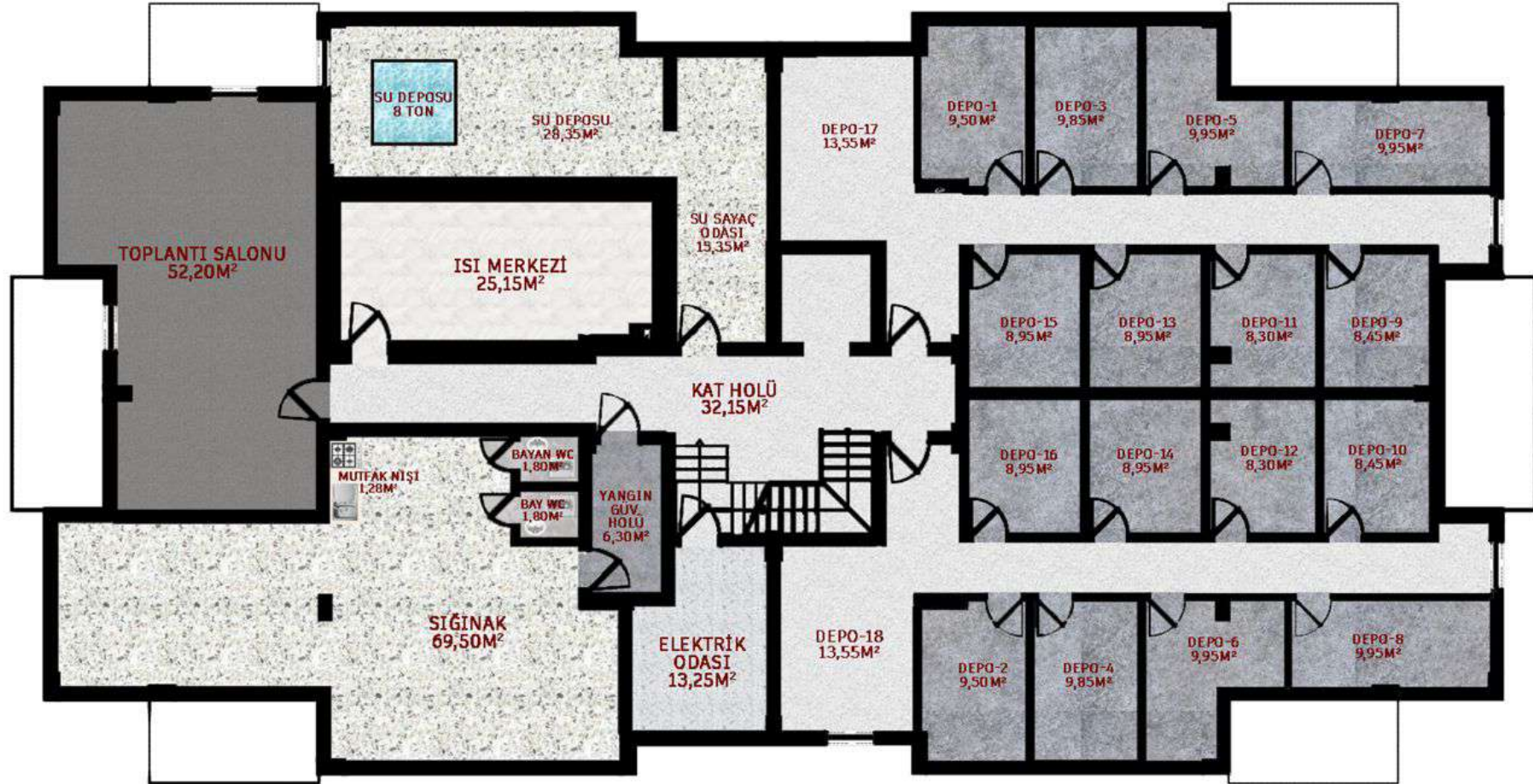
BODRUM KAT PLANI
